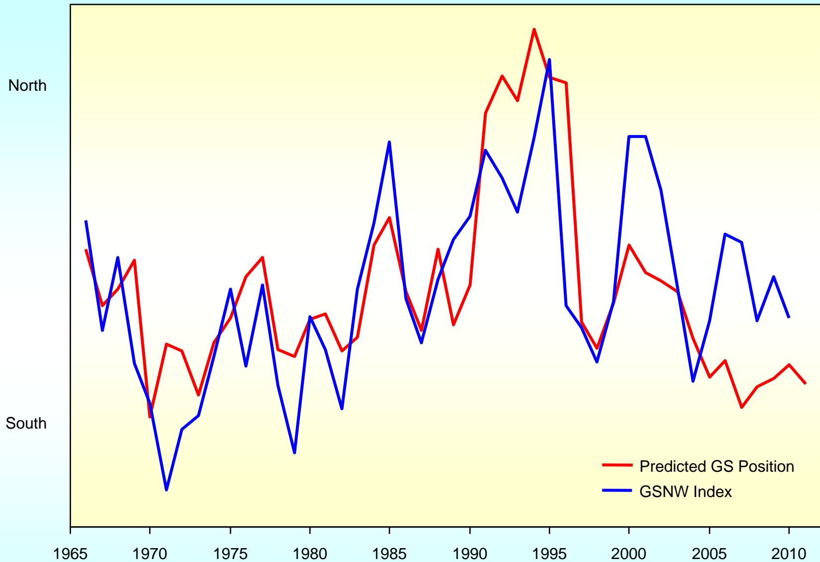
Values of the GSNW Index compared with predictions (1966 to 2011) of the model of Taylor and Gangopadhyay (J. Geophys. Res., 106, C7, 13849-13860, 2001). The calculation used the parameter values in this paper, with a 2 km surface layer and a one year delay in the NAO index. The model predicts a southerly position during 2011.
