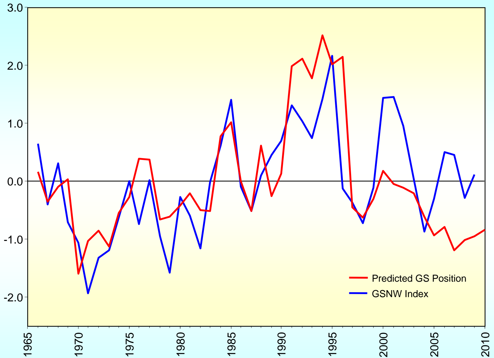
Values of the GSNW Index compared with predictions (1966 to 2010) of the model of Taylor and Gangopadhyay (J. Geophys. Res., 106, C7, 13849-13860, 2001). The calculation used the parameter values in this paper, with a 2 km surface layer and a one year delay in the NAO index. The model predicts a southerly position during 2010.
